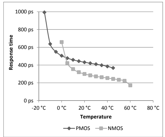
Figure 5: Response time in function of temperature (6 heads, Q_f = 2 fC, t_f = 5 ps)
